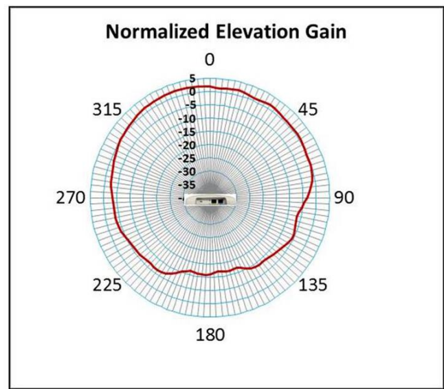
5 GHz Elevation
